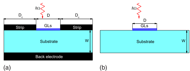
FIG. 1. (Color online) Schematic views of the device structures under consideration: (a) with a SLW and (b) with a DW.
