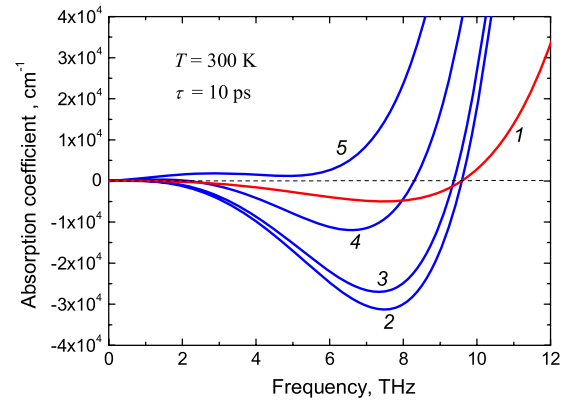
Figure 6. Frequency dependences of SP absorption for SGL structures with different substrate refractive indices n : 1— n = 1.0 , 2— n = 3.4 , 3— n = 3.4 + i0.01 , 4— n = 3.4 + i0.05 , and 5— n = 3.4 + i0.1 ( T = 300 \text{ K} , \varepsilon_F^T = 20 \text{ meV} ).
