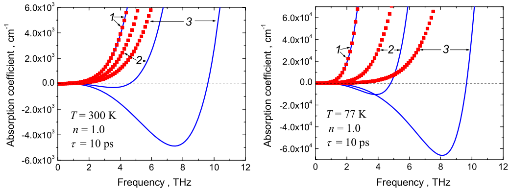
Figure 4. Frequency dependences of the SP absorption coefficient 2 \text{Im}(q) in an SGL structure at T = 300 \text{ K} (left panel) and T = 77 \text{ K} (right panel) and for different quasi-Fermi energies (1— \varepsilon_F^T = 0 \text{ meV} , 2— \varepsilon_F^T = 10 \text{ meV} , and 3— \varepsilon_F^T = 20 \text{ meV} ). The markers show the dependences for equilibrium electron–hole systems calculated using the derived formulas as well as using [13] for intrinsic and doped SGL structures.
